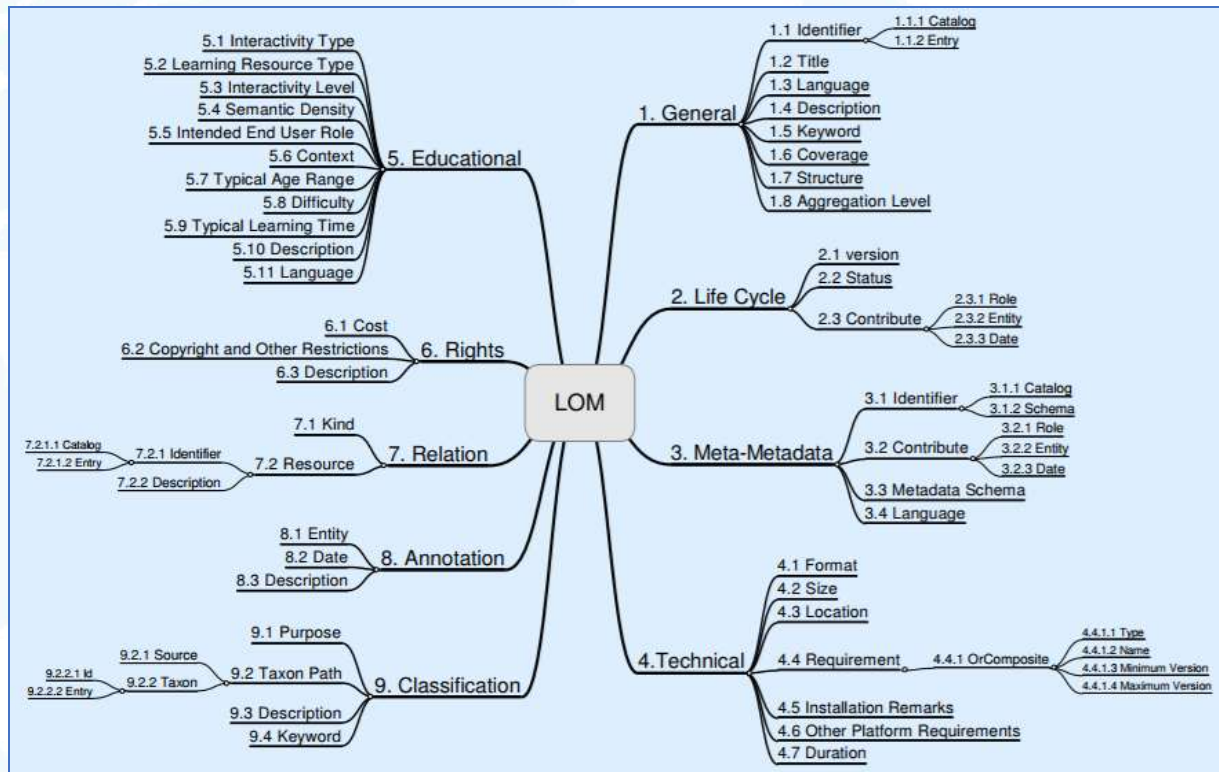
Figure 4. A schematic representation of the hierarchy of elements in the LOM data model (Barker, 2005, p. 2)
