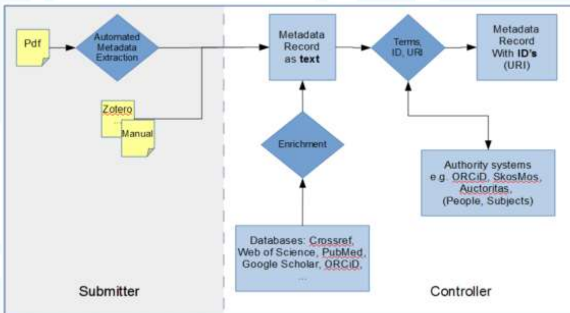
Figure 8: Extracting and enriching metadata from research documents
