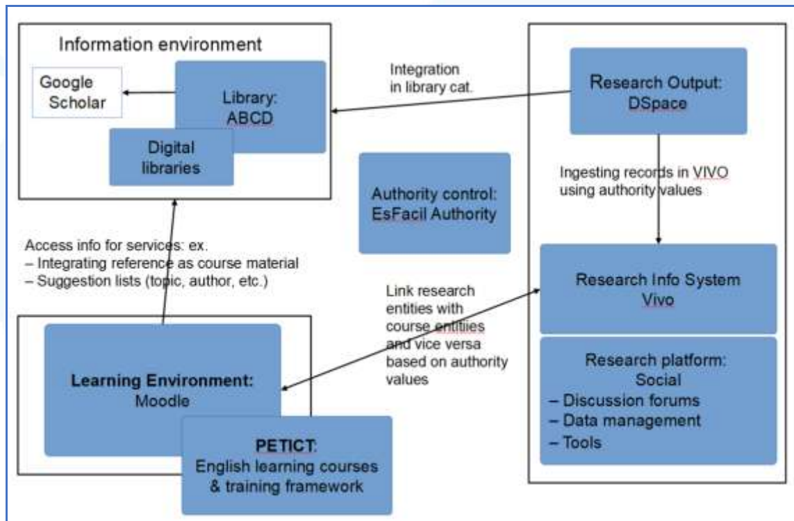
Figure 1. The VLIREC Cuba Virtual Research, Information and Education Network
