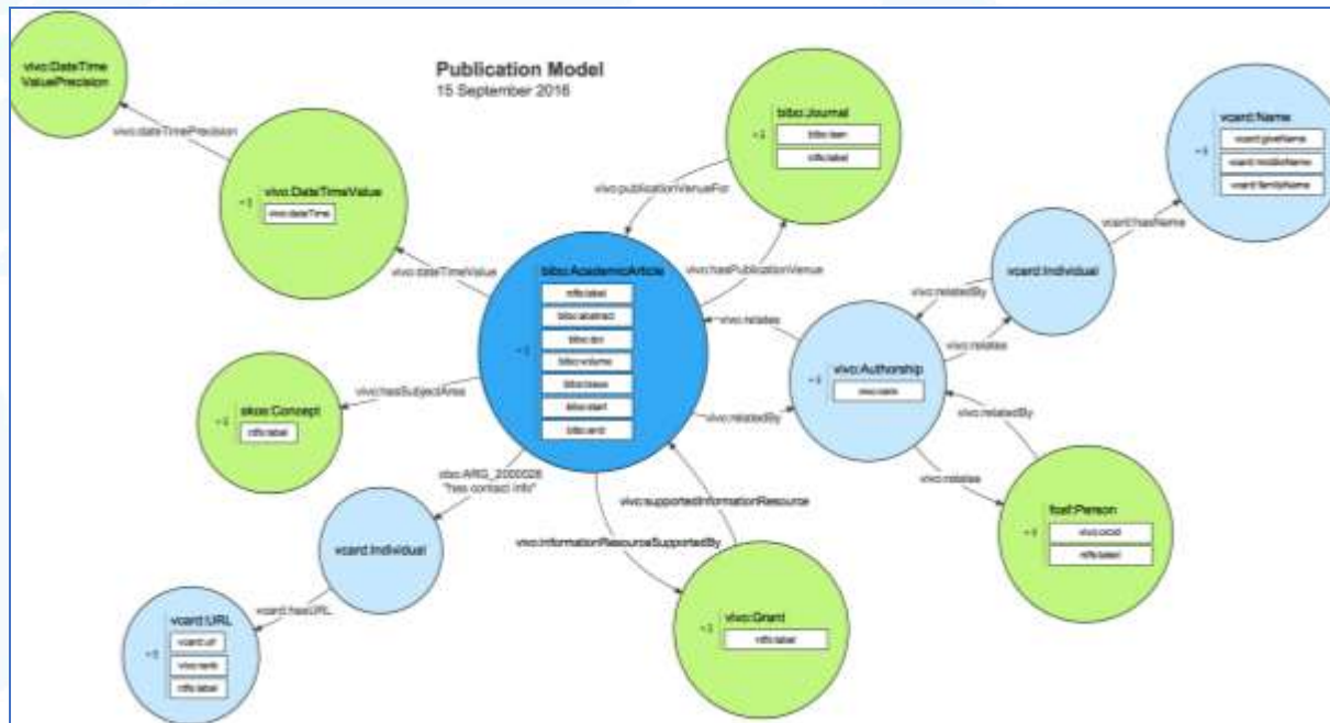
Figure 4. Entities of the publication model of VIVO ( https://wiki.duraspace.org/display/VIVODOC19x/Publication+Model )
